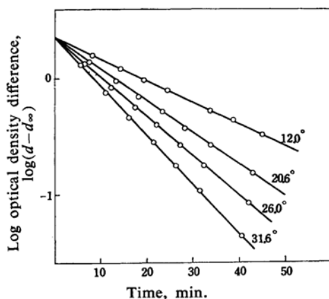
Fig. 6. Hydrolyzation reaction of
