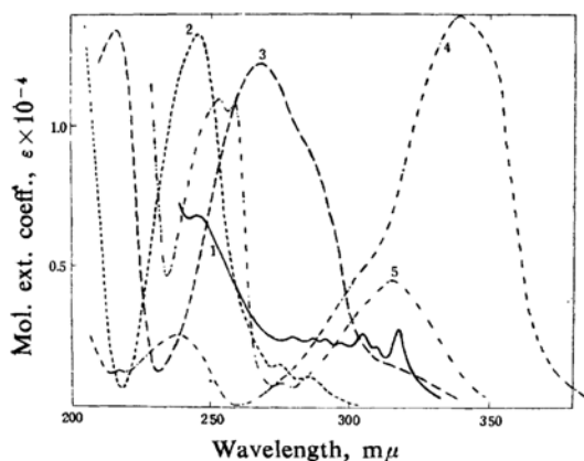
Fig. 3. Spectra of aliphatic anils in n -heptane:
