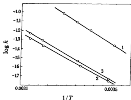
Fig. 7. Temperature dependences of
