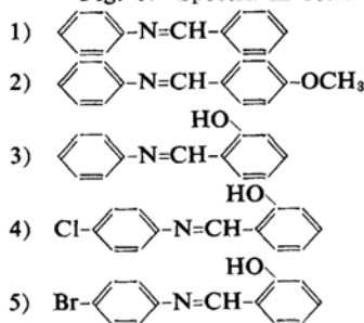
Fig. 8. Spectra in solid states,
