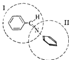
Fig. 1. Assumed structure of benzylideneaniline.
