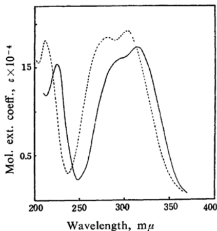
Fig. 4. Spectra of 1) c1ccc(cc1)/N=CH/c2ccc(O)cc2 and 2) c1ccc(cc1)/N=CH/c2ccc(OC)cc2 in C 2 H 5 OH.
