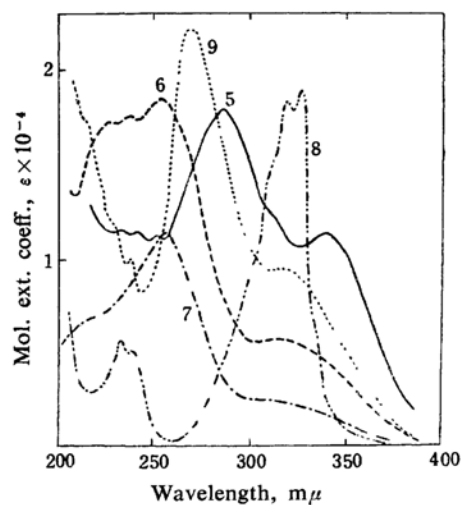
Fig. 2(B). Spectra of anils in n -heptane:
