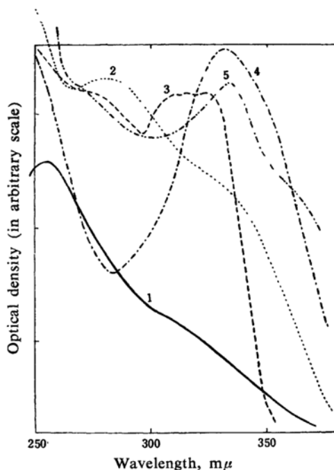
Fig. 8. Spectra in solid states,
