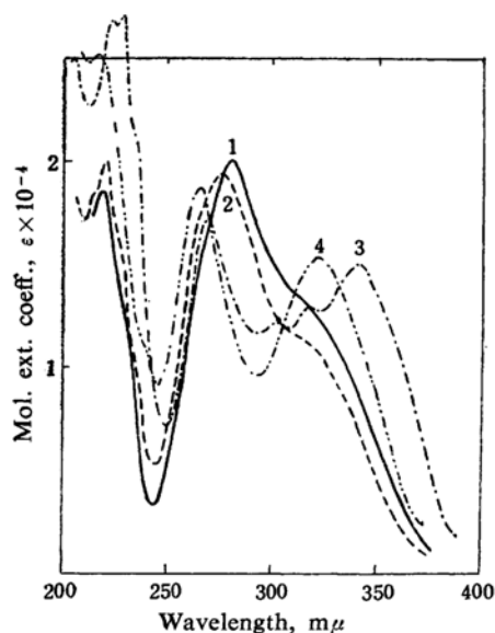
Fig. 2(A). Spectra of anils in n -heptane.
