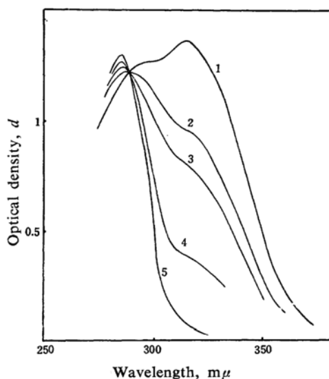
Fig. 5. Time-dependence of the spectrum of
