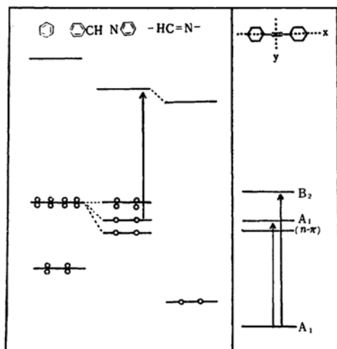
Fig. 9. Energy level diagrams of planar benzylideneaniline molecule.
